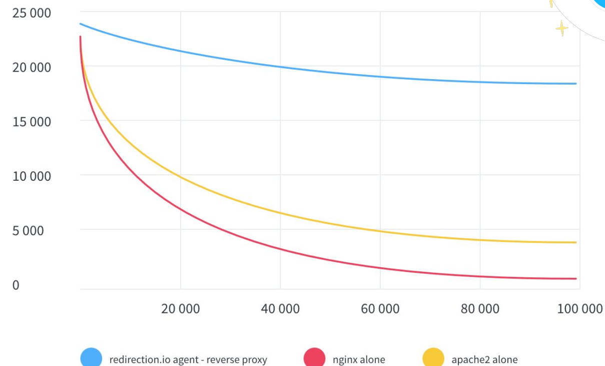
req/s depending on the number of rules
